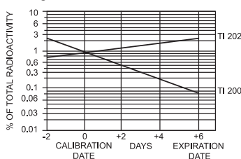
Figure 1. Radionuclidic Contaminants
